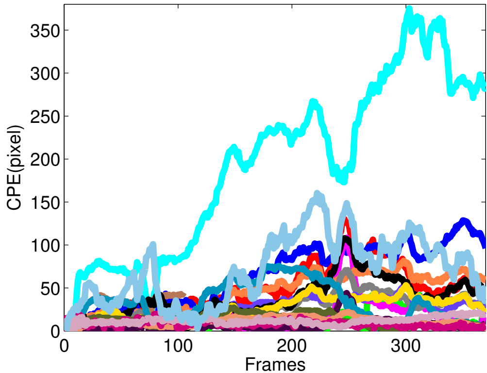
Center Positioning Error
