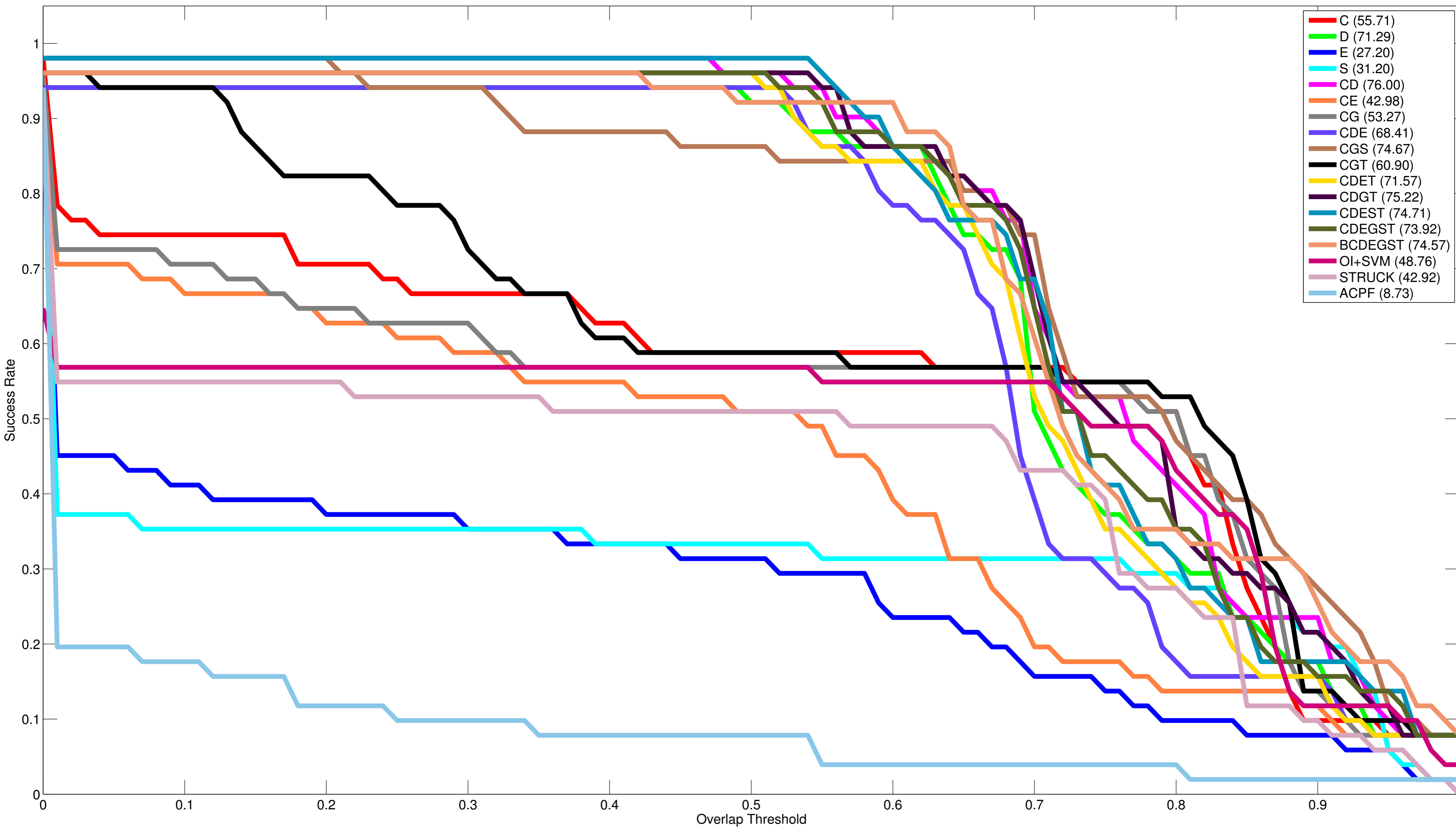
Success Plot
