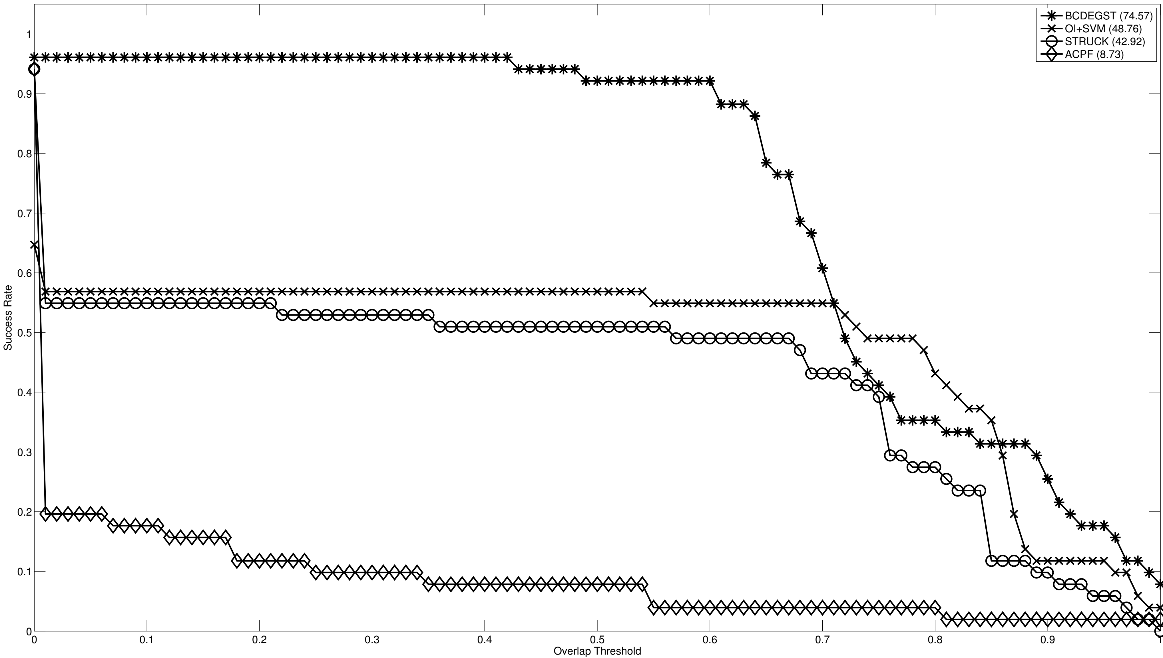
Success Plot
